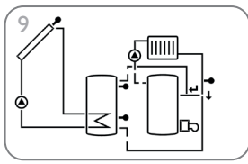
Solar system with heating circuit return preheating (page 42)
