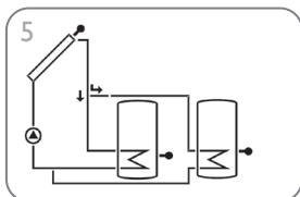
Solar system with 2 stores and valve logic (page 27)
